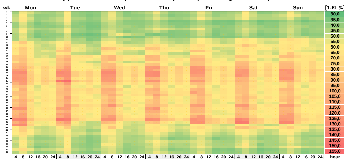
Appearance of RL penetration by RES (including must run)
