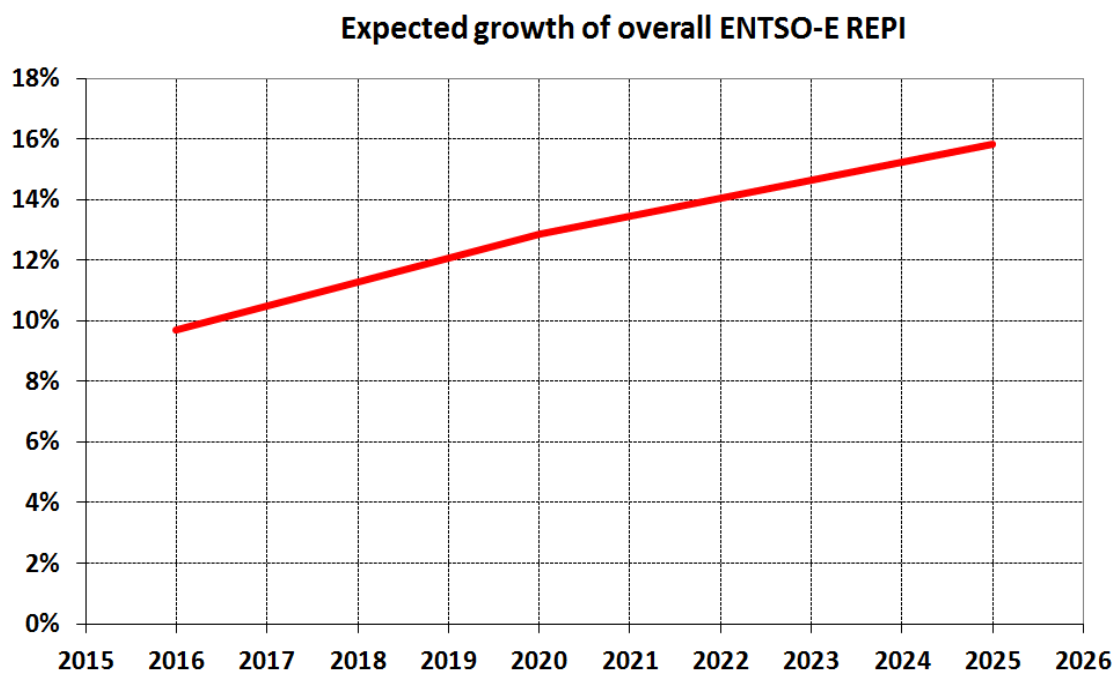
Figure 5.4.2–Expected growth of the RES energy penetration index–REPI
