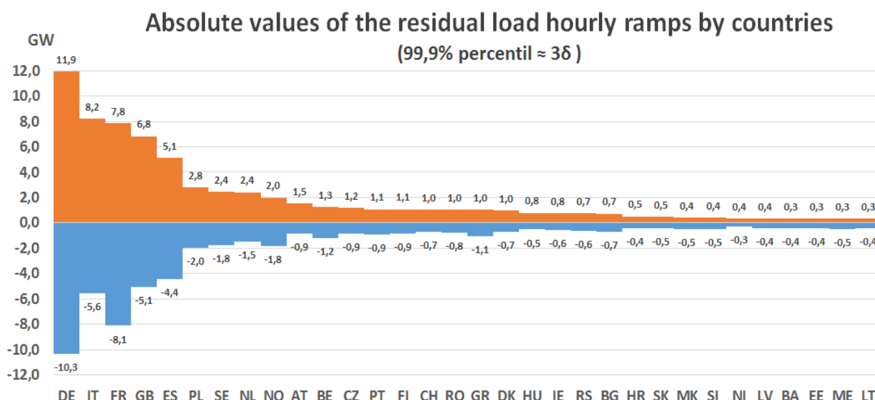
Figure 5.5.2— 3\sigma distribution of the absolute residual load ramp by ENTSO-E countries calculated for year 2020 Scenario B.
